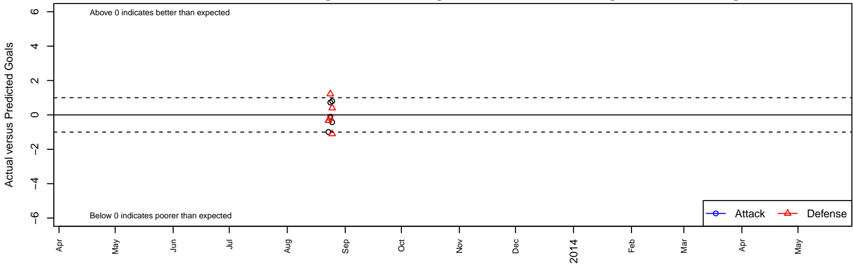
Santa Rosa United Milan B01 Dots are actual minus expected GF (blue circles) and GA (red triangles). Blue line is smoothed change in attack strength. Red is smoothed change in defense strength.
